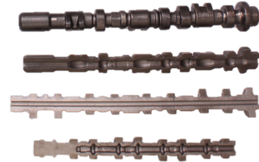
Solid, hollow and profiled hollow core (using glass/sand core) Special profiled hollow and Variable valve-lift camshafts
