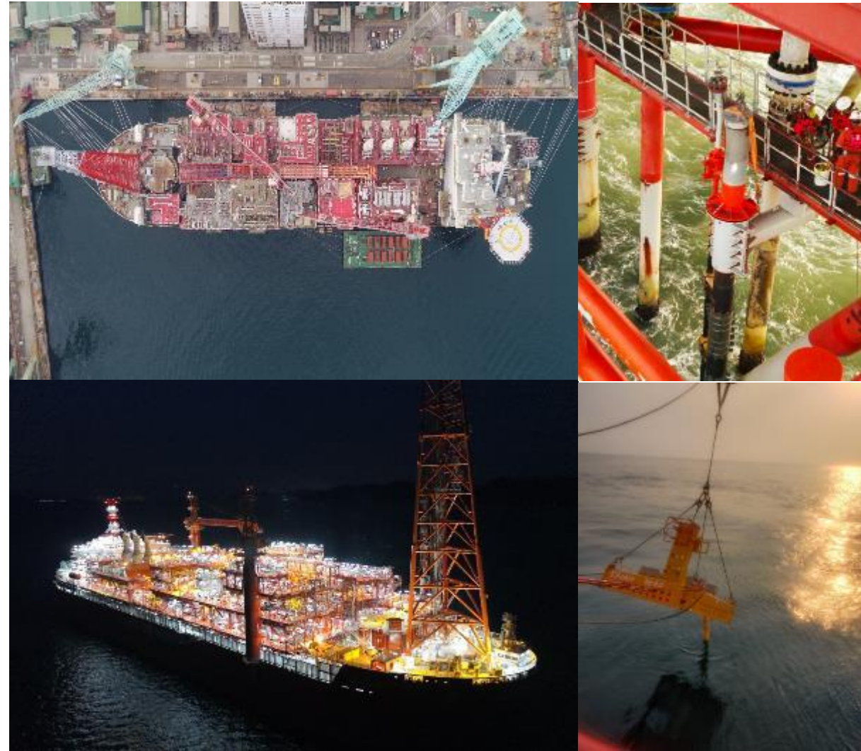
MJ: FPSO & Field Installation Pictures
