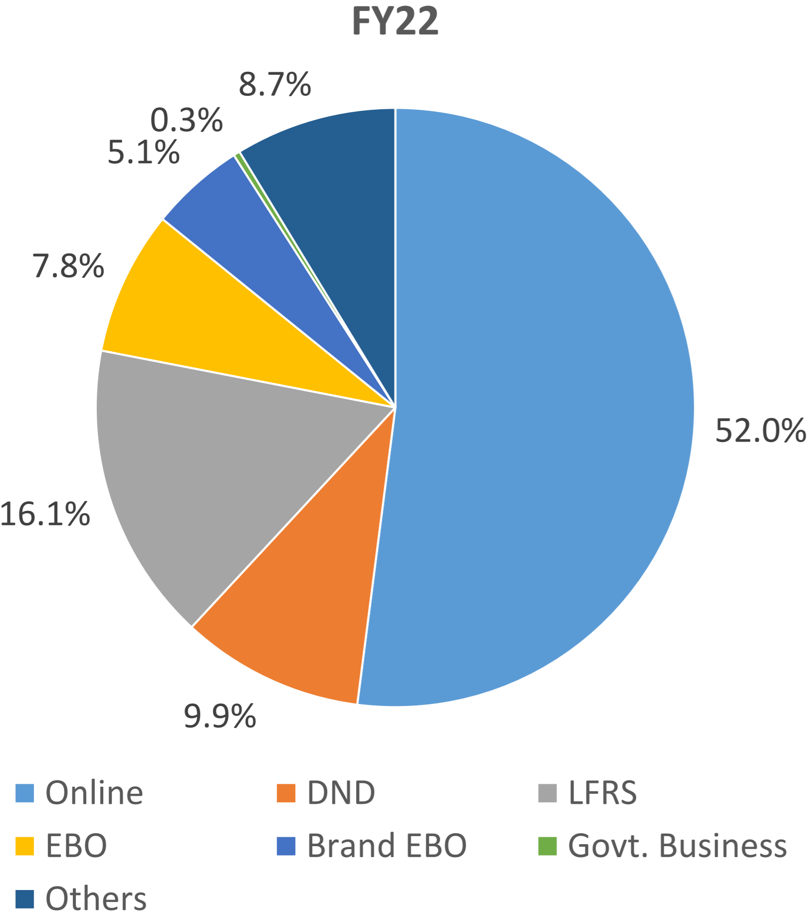
Channel Contribution
