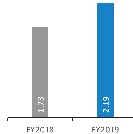
Current Ratio
