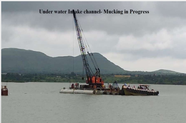
Irrigation Work in progress, Bhama, Pune
